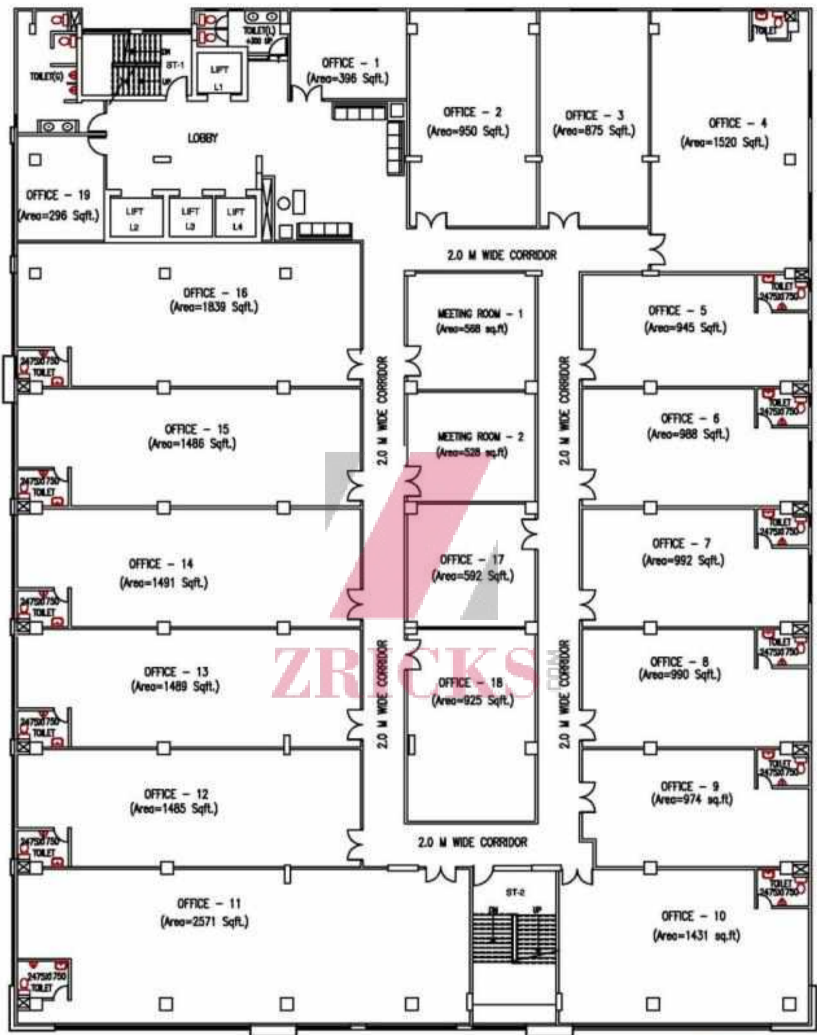
SIXTH FLOOR PLAN
